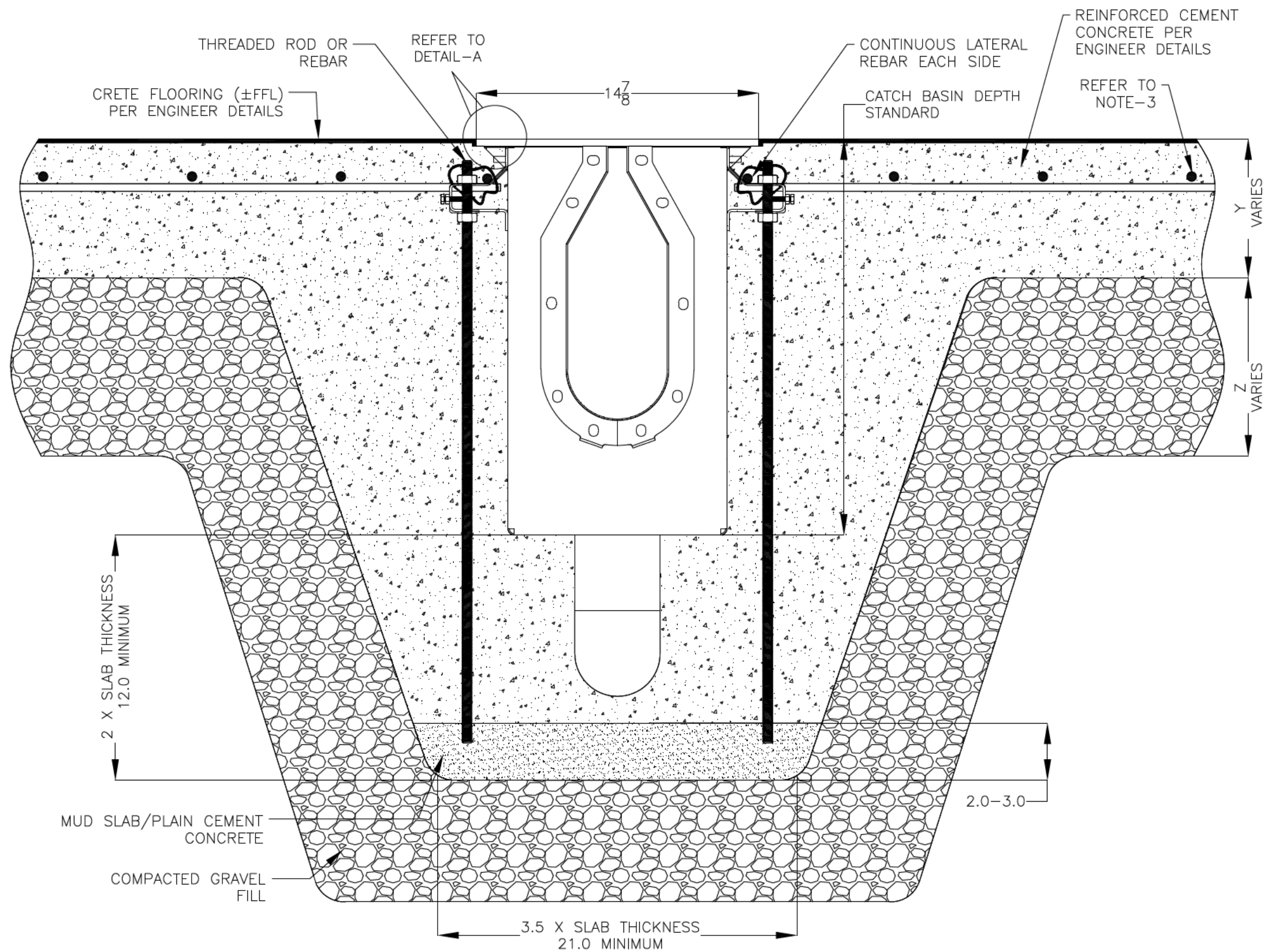
12X12X20 CATCH BASIN INSTALLATION DETAILS
