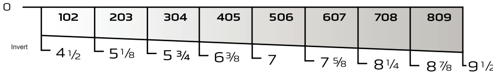
TYPICAL MODULAR LAYOUT OF A 4000 SERIES LANDSCAPE SLOT DRAIN® (Sections fit together as illustrated below)
