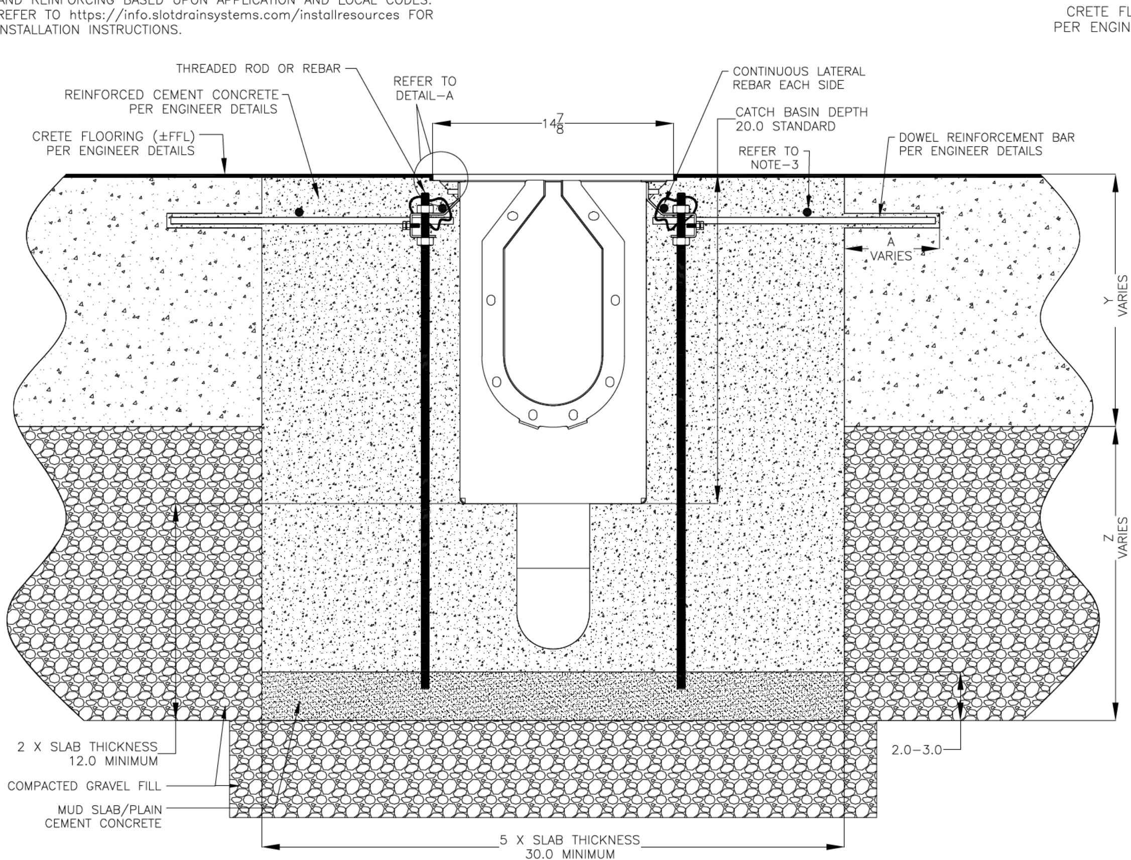
12X12X20 CATCH BASIN INSTALLATION DETAILS
