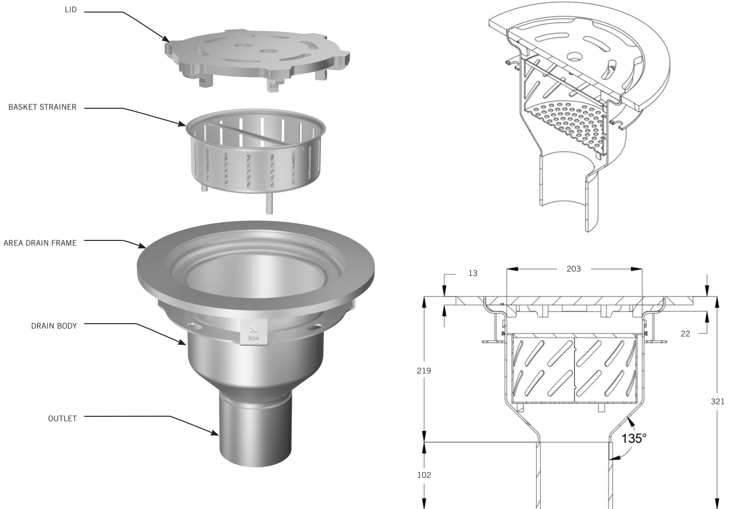
TYPICAL PROFILE OF A FOOD SAFE AREA DRAIN - CONE SYSTEM
