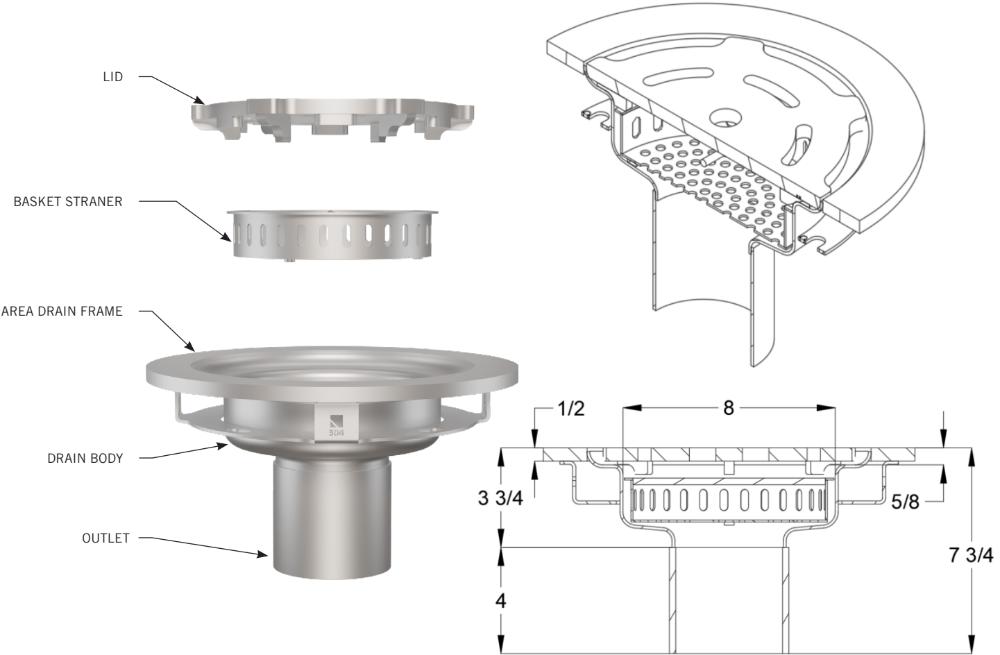
TYPICAL PROFILE OF A FOOD SAFE SHALLOW AREA DRAIN - ROUND SYSTEM
