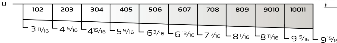
TYPICAL MODULAR LAYOUT OF A 6000 PLUS SERIES SLOT DRAIN ® (Sections fit together as illustrated below)
